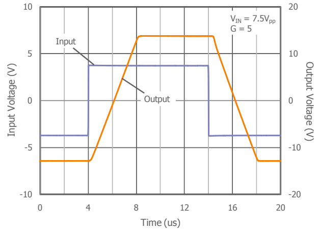
Figure 5. Overdrive Recovery
