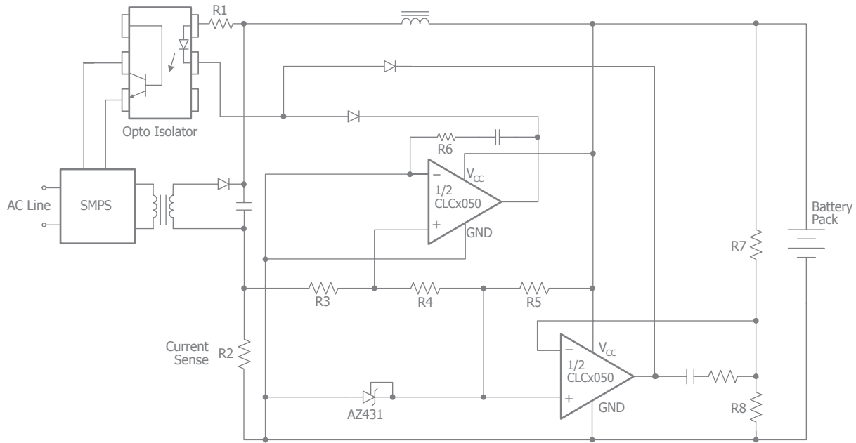
Figure 18. Battery Charger
