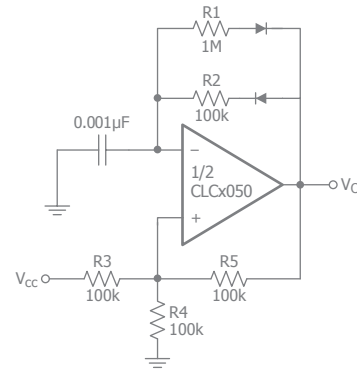
Figure 23. Pulse Generator
