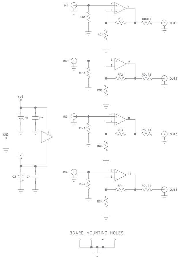
Figure 15. CEB018 Schematic
