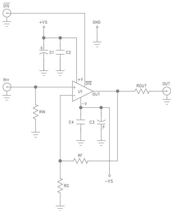
Figure 9. CEB002 Schematic
